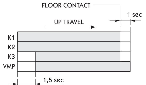
ALARM CONTROL (inductances - motor)
