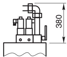
application of shut off valve for power unit in machine room enclosure
